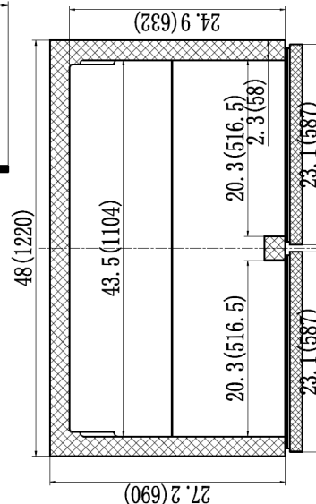
PLAN VIEW
